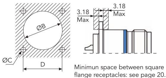
Type 2 Square flange receptacle
