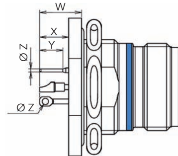
Type 7: Jam nut receptacle
