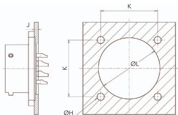
Panel cut-out
