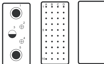
Insert 5W2 (2) Size 16 Contacts (40) Size 22 Contacts (1) Size 12 Contact (2) Size 5 Coax Contacts
