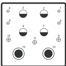
Insert 13W2 (4) Size 12 Contacts (3) Size 16 Contacts (5) Size 20 Contacts (2) Size 5 Coax Contacts
