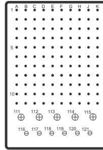
Insert 121 (110) Size 22 Contacts (6) Size 20 Contacts (5) Size 16 Contacts
