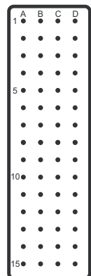
Insert 60 (60) Size 22 Contacts
