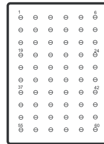
Insert 60 (60) Size 20 Contacts
