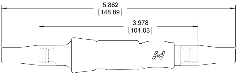
PLUG & CABLE RECEPTACLE MATED PAIR with strain relief
