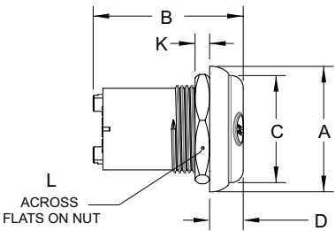
[E] RECEPTACLE
