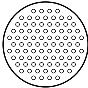
85x SPRING PROBE CONTACTS (Custom Mating Face)
