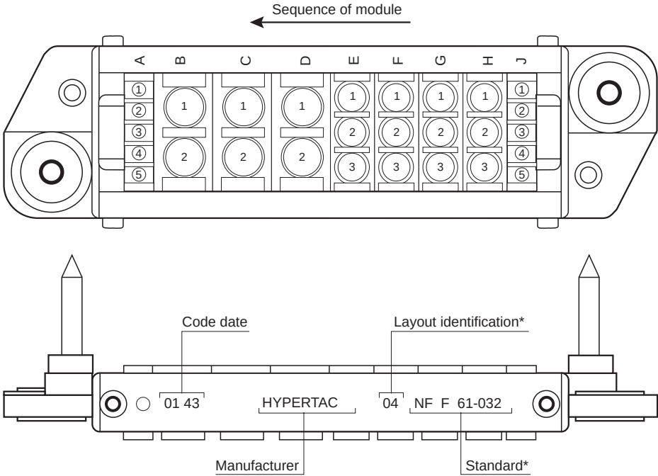
PLUG CABLING SIDE VIEW
