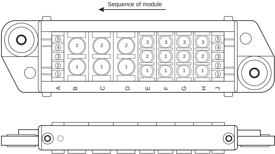
RECEPTACLE CABLING SIDE VIEW
