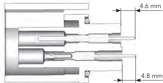
UTL7 male
