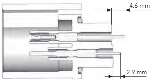
UTL7 female
