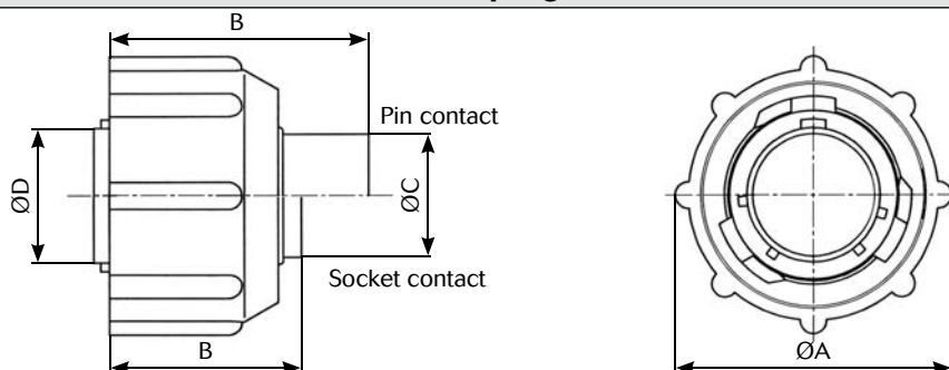
Cable plug - UTP6
