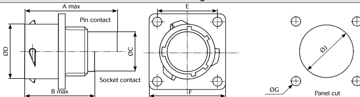
Panel mounting - UTP0
